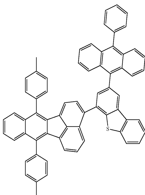
17 -continued
