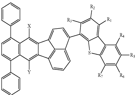
Formula X
