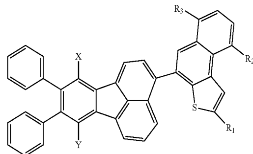
Formula X
