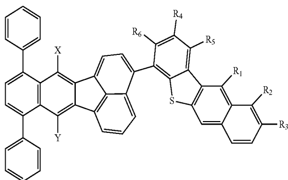
Formula XIII
