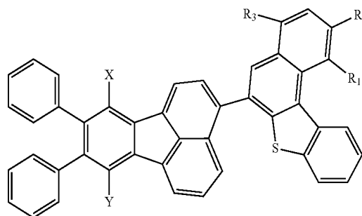
Formula VIII
