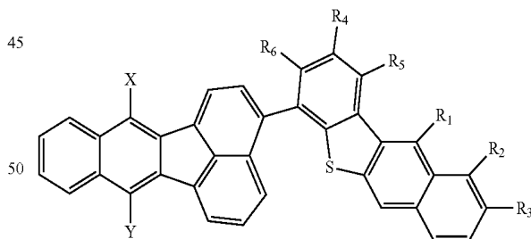
Formula V
