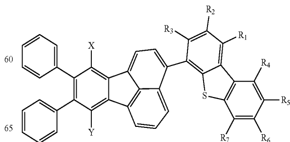
Formula VI
