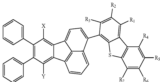
Formula VII
