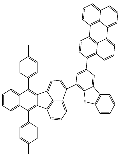
19 -continued
