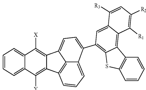
Formula IV
