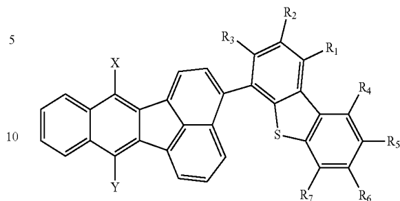
Formula III
