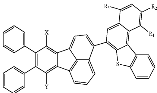
Formula VII
