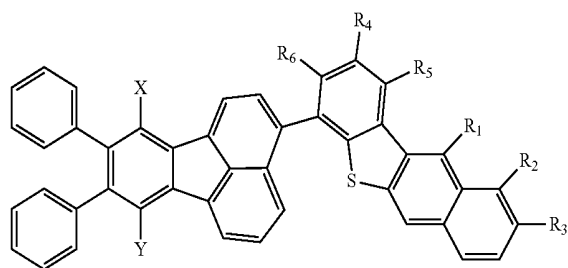
Formula VIII
