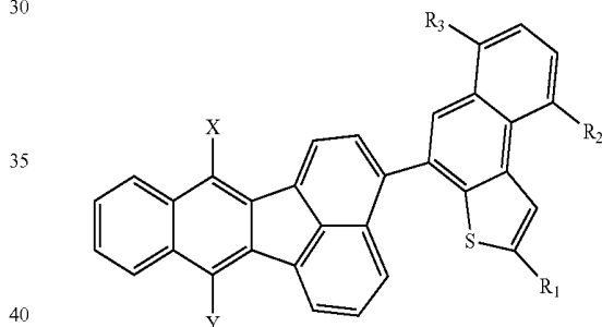
Formula IV
