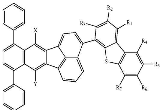
Formula X
