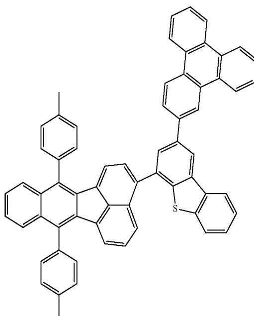
18 -continued
